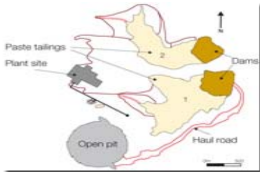
Proposed infrastructure (Click to enlarge)
